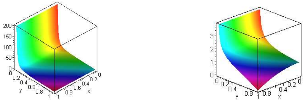
Fig. 3. The distribution of the normalized flux density b(x, t) at different times t=0.1, 0.2 for n=1, q=1 .
